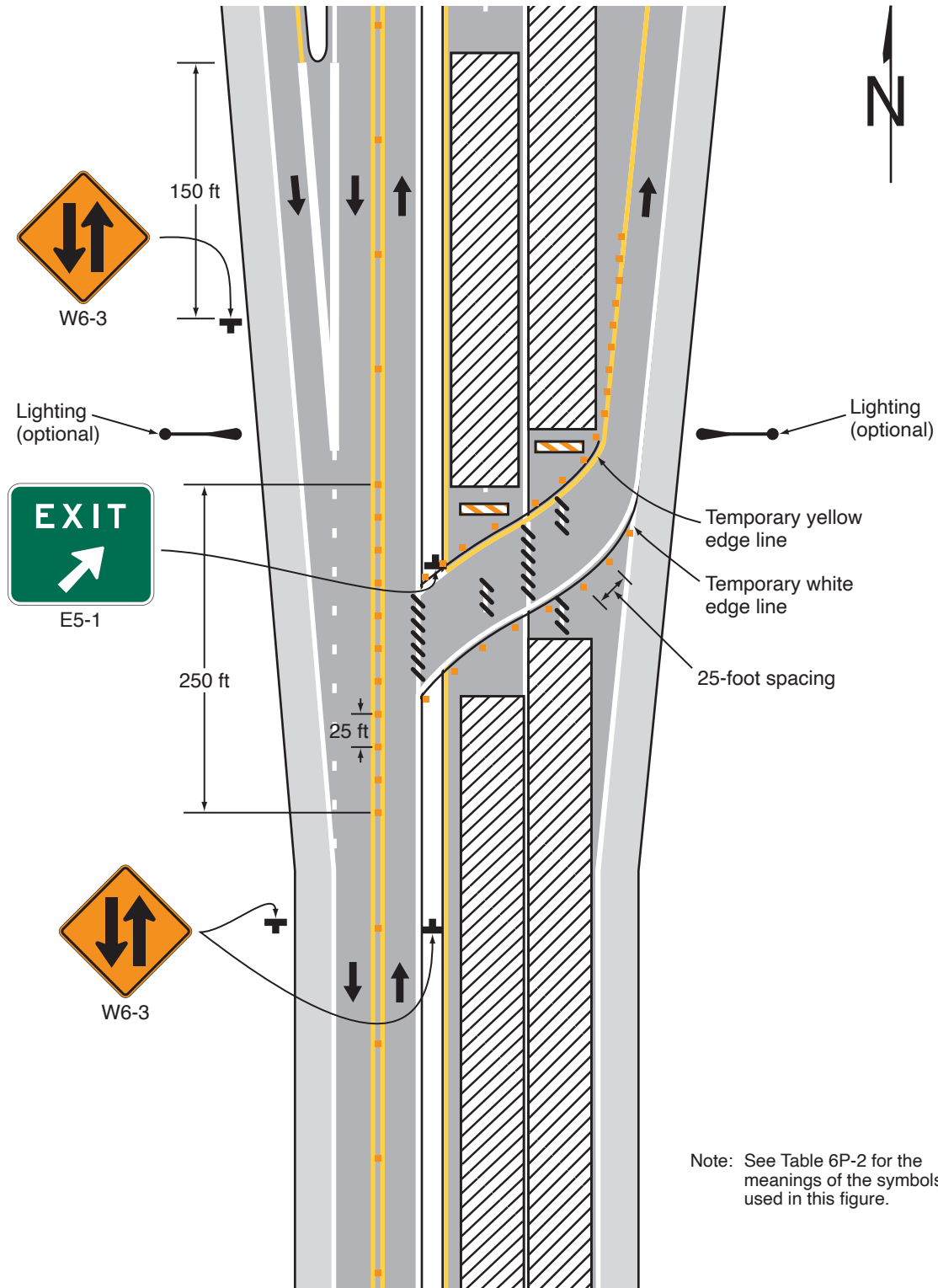
Figure 6P-41. Median Crossover for an Exit Ramp (TA-41)
