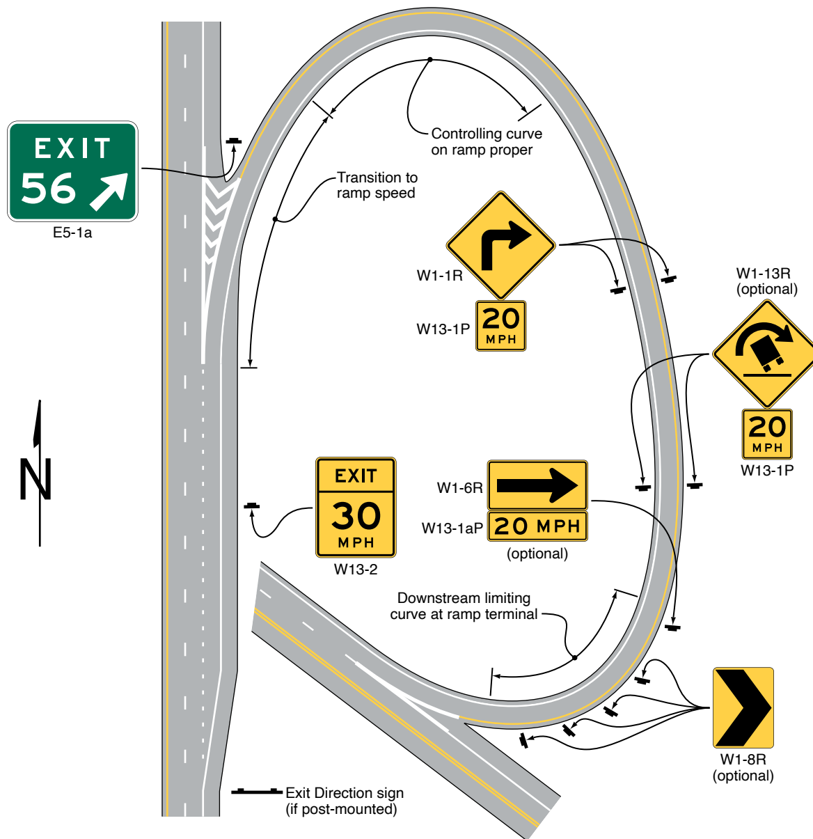
Figure 2C-3. Examples of Exit Ramp Advisory Speed and Other Warning Signs (Sheet 2 of 5)
