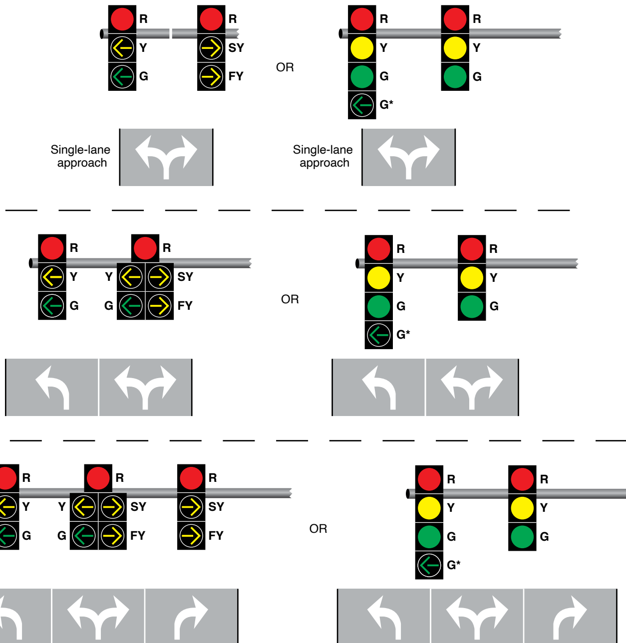
Figure 4F-15. Signal Indications for Approaches with a Combined Left-Turn/Right-Turn Lane and No Through Movement (Sheet 2 of 3)
