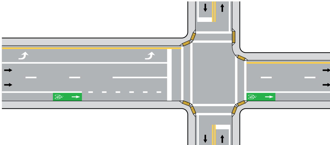
C – Applied approaching and departing an intersection
