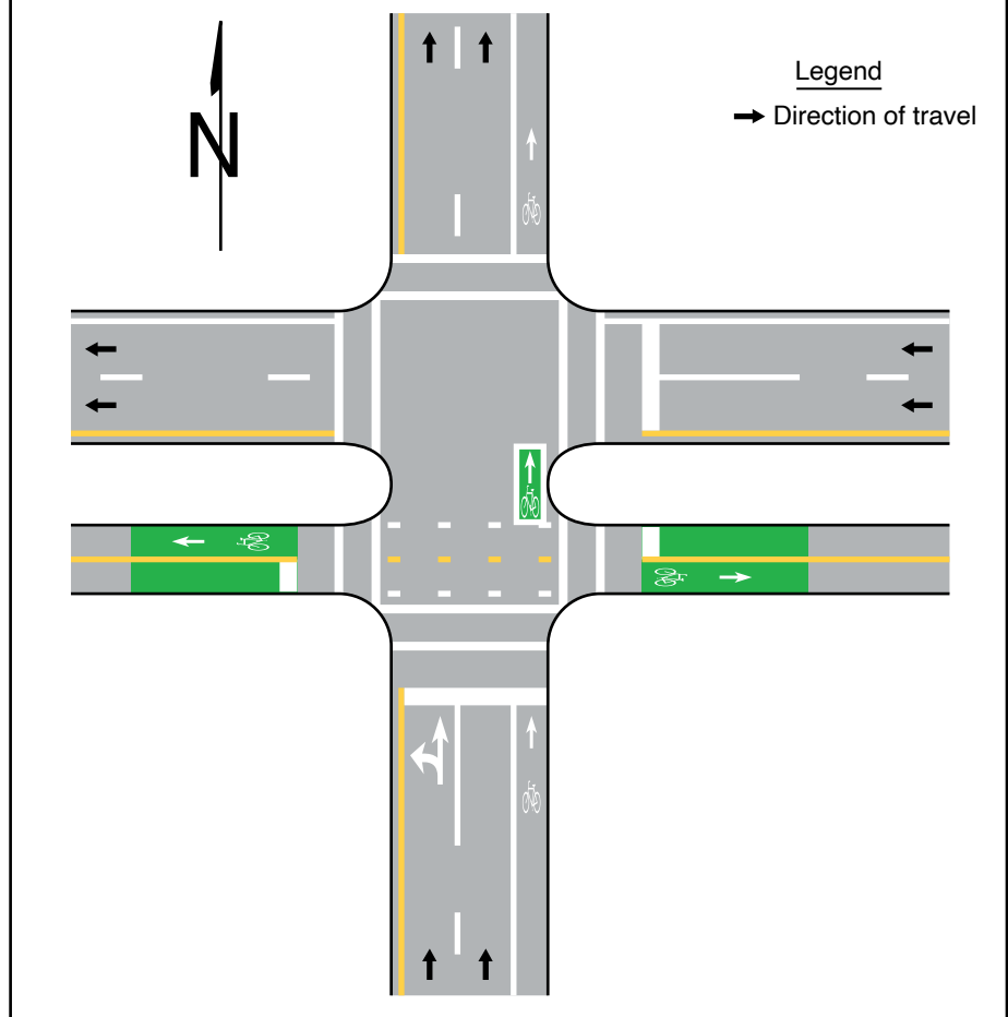
Figure 9E-11. Example of a Two-Stage Turn Box Location at an Intersection with a Two-Way Bikeway
