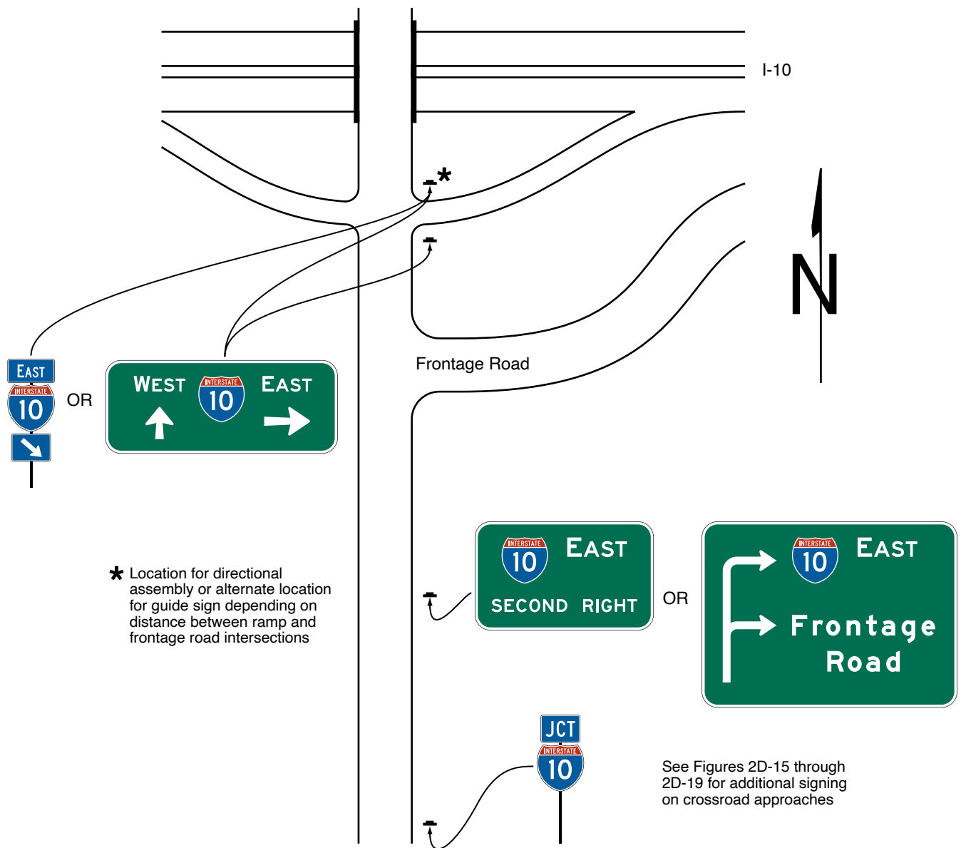
Figure 2D-20. Example of Crossroad Guide Signing for an Entrance Ramp with a Nearby Frontage Road
