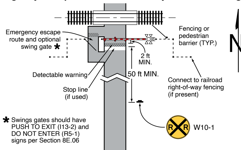
Figure 8E-6. Example of an Automatic Pedestrian Gate and an Emergency Escape Route at a Pathway Grade Crossing
