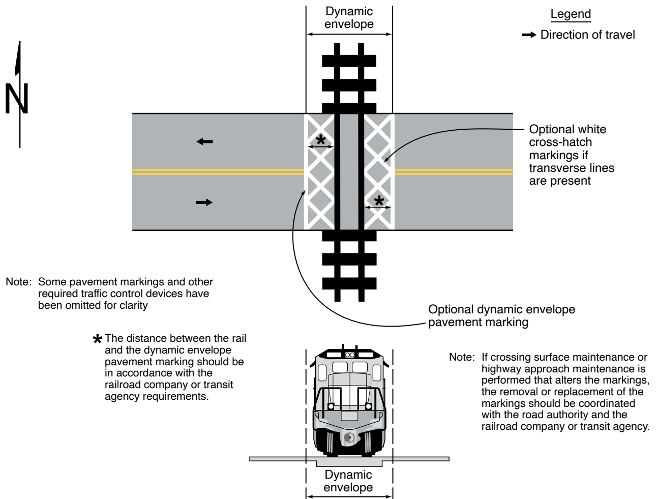
Figure 8C-3. Example of Dynamic Envelope Pavement Markings at Grade Crossings
