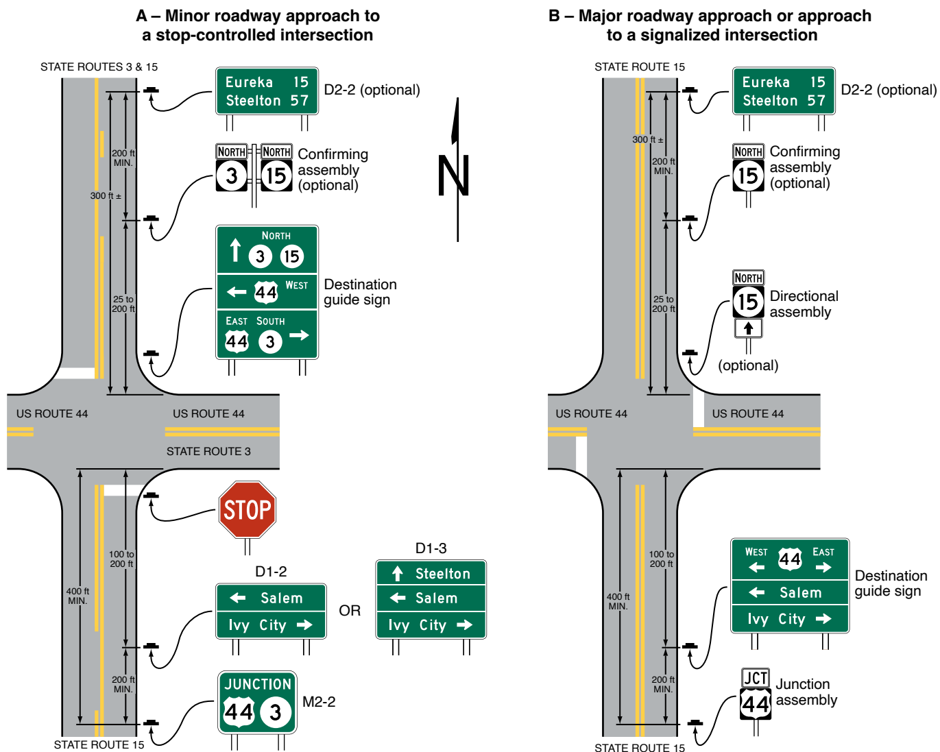
Figure 2D-7. Examples of Consolidation of Route Sign Assemblies into Guide Signs (Sheet 1 of 2)
